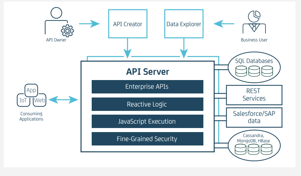
CA Live API Creator
